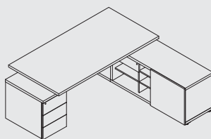
MIT1KD 2497 | 2080 | 740 98 1/4" | 81 7/8" | 29 1/8"
