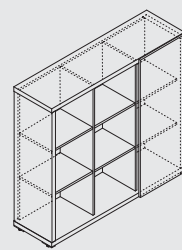
MIT7 1400 | 422 | 1280 55 1/8" | 16 5/8" | 50 3/8"
